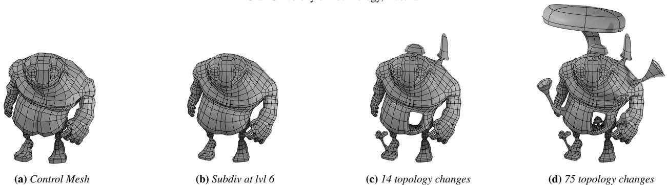
Figure 1: A set of modeling operations applied to the control mesh of the BigGuy model (a). In total, a sequence of 75 connectivity changing operations are performed from (b) to (d). The current industry standard, OpenSubdiv, needs serial preprocessing after each topology change. These delays sum up to a two-minute idle time till (c) and an eleven-minute delay till (d). Using our subdivision-specialized linear algebra kernels, a modeler performs the whole sequence within two minutes with a consistent 30 fps preview of the subdivision surface at level six.
